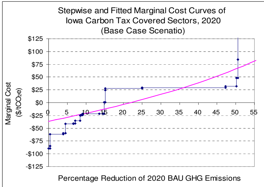
Figure 1. Stepwise and fitted marginal cost curves of Iowa carbon tax-covered sectors (base case scenario), 2020
