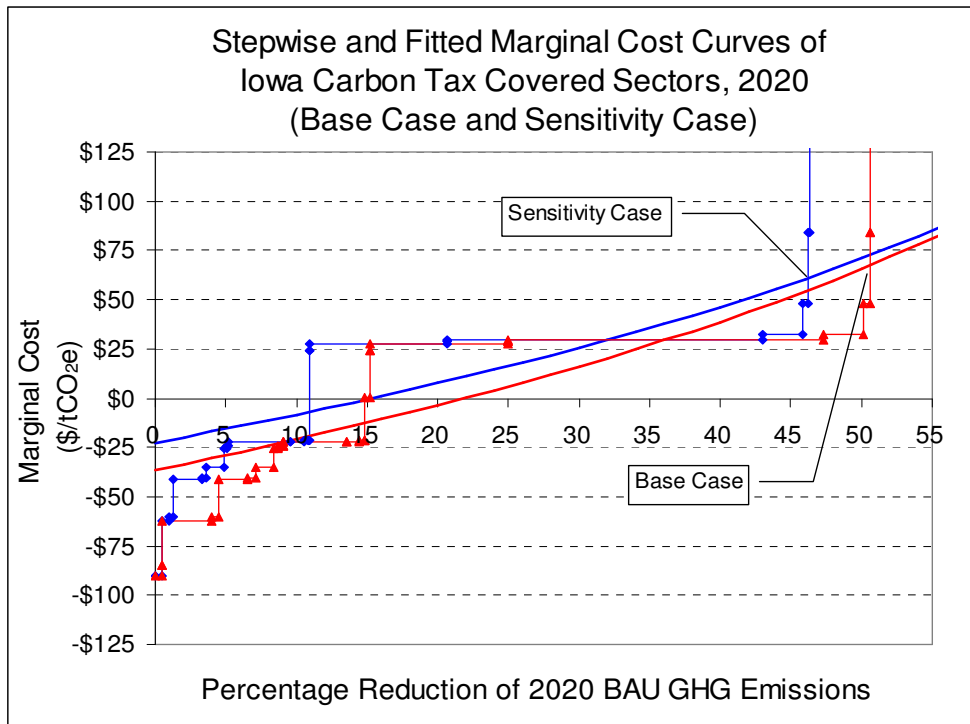
Figure 2. Stepwise and fitted marginal cost curves of Iowa carbon tax-covered sectors (base case and sensitivity case), 2020
